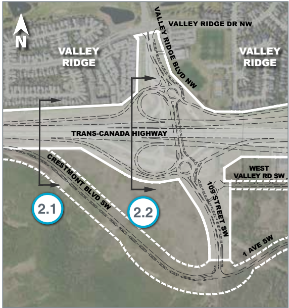
Plan View
